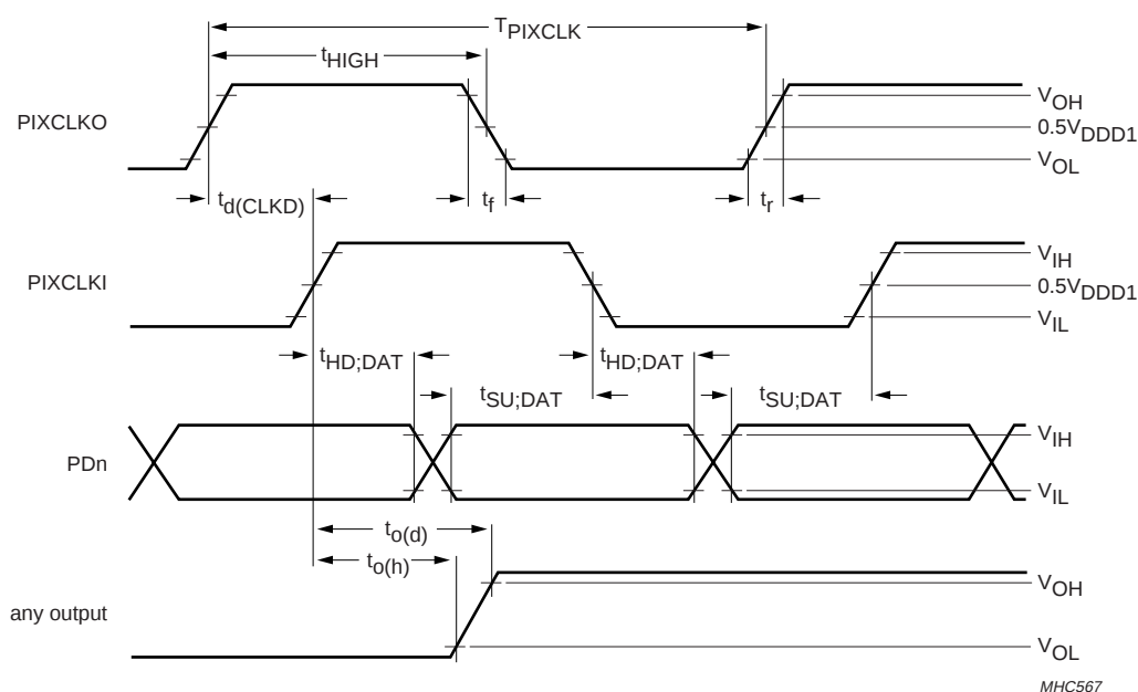
Fig.11 Input/output timing specification.
